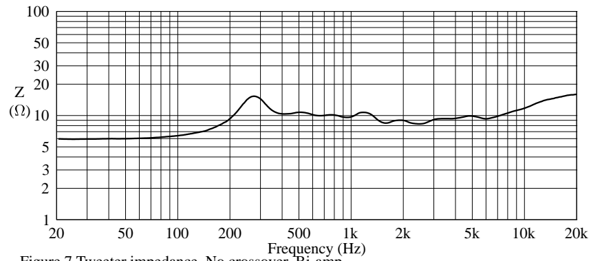
Figure 7 Tweeter impedance, No crossover, Bi-amp
