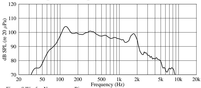
Figure 8 Woofer, No crossover, Bi-amp
