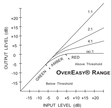
OverEasy® compression threshold and LEDs.
