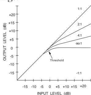
Behavior of the 162SL's Compression control
