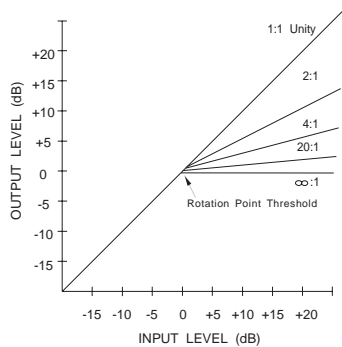
Hard knee compression threshold point.
